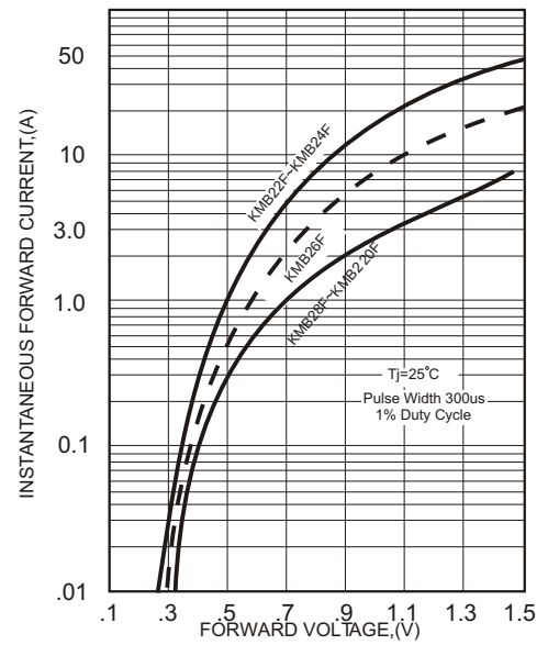
FIG.2-TYPICAL FORWARD CHARACTERISTICS
