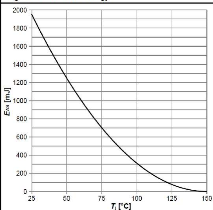
Diagram 12: Avalanche energy
