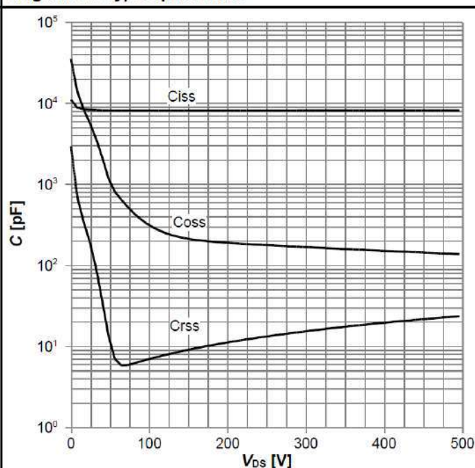
Diagram 14: Typ. capacitances
