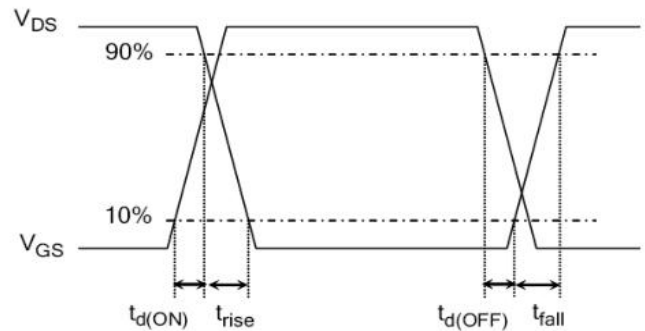
Figure 20. Resistive Switching Waveforms
