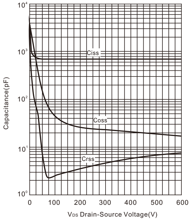
Fig12. Capacitance Characteristics
