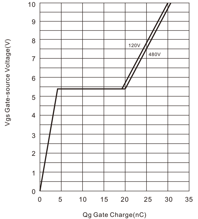
Fig13. Gate Charge
