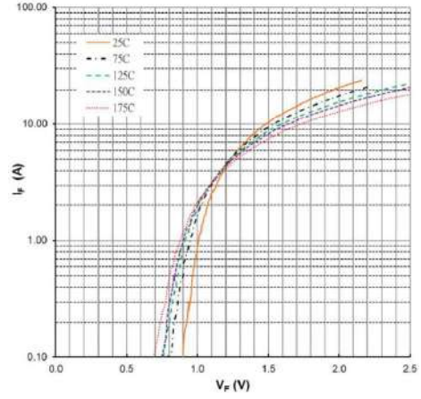
Figure 2. Forward Characteristics
