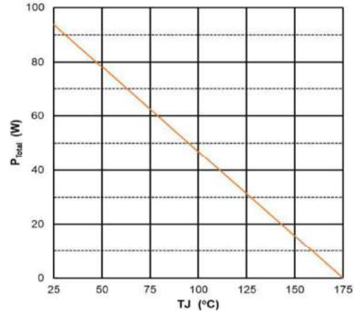
Figure 4. Power Derating
