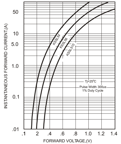
FIG.2-TYPICAL FORWARD
