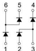
BAT54BRW
