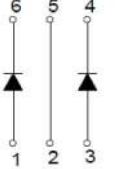
BAT54JW
