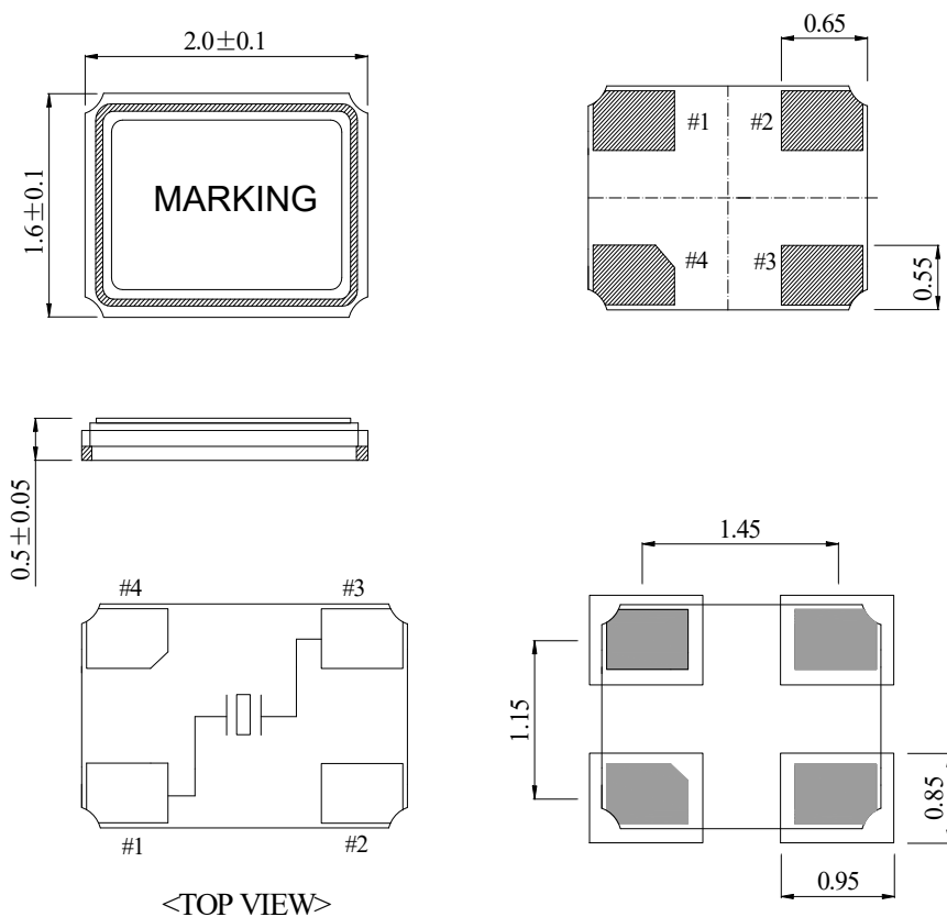
Recommended Solder Pad Layout:
