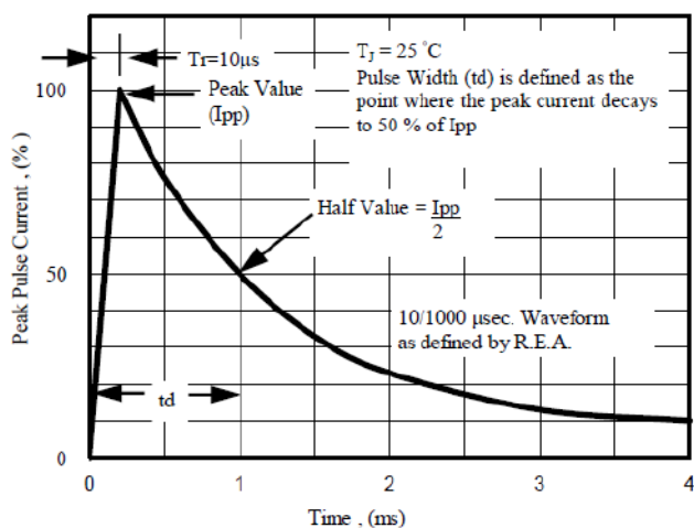
Fig. 5 - Pulse Waveform
