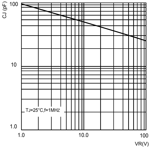
FIG.3-TYPICAL JUNCTION CAPACITANCE
