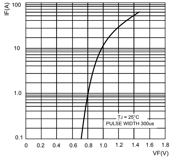
FIG.4-TYPICAL FORWARD CHARACTERISTICS
