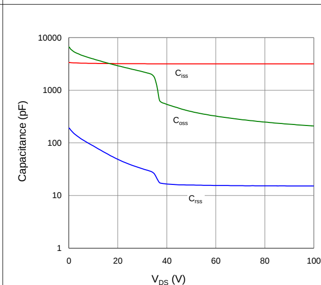
Figure 8. Typical Capacitance vs. Drain-to-Source Voltage
