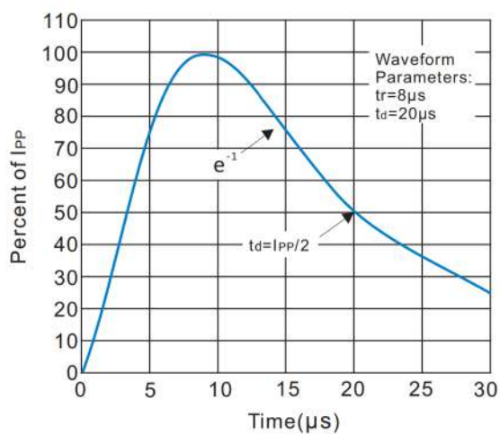
Fig.2 Pulse Waveform
