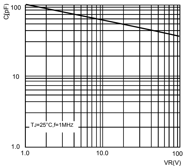
FIG.5-TYPICAL JUNCTION CAPACITANCE
