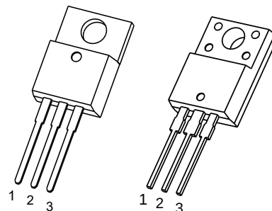
TO-220AB
