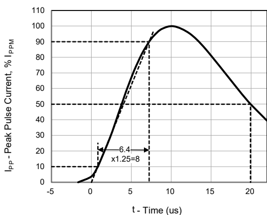
Fig.3 - 8/20us Pulse Waveform
