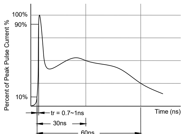
Fig4. ESD Clamping (-8KV Contac per IEC61000-4-2)
