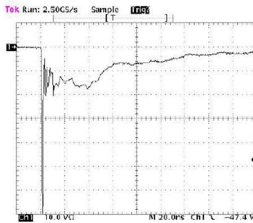
Fig4. ESD Clamping (-8KV Contac per IEC61000-4-2)
