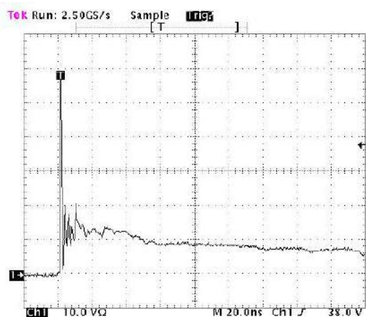
Fig3. ESD Clamping (+8KV Contac per IEC61000-4-2)
