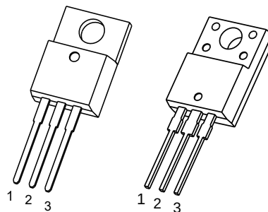
TO-220AB ITO-220AB
