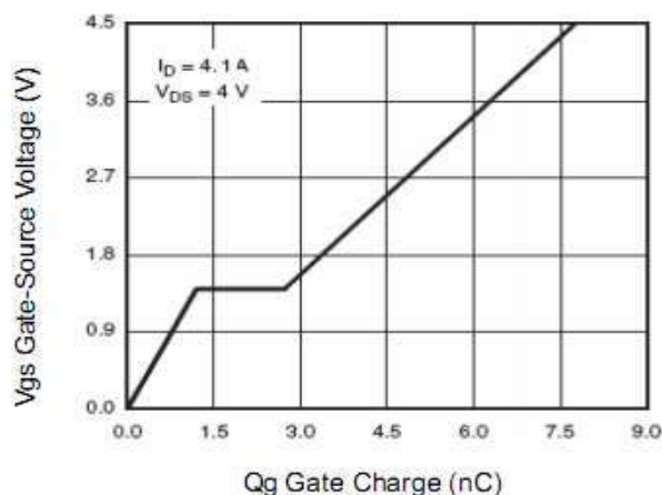
Figure 11 Gate Charge
