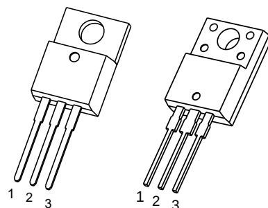
TO-220AB
