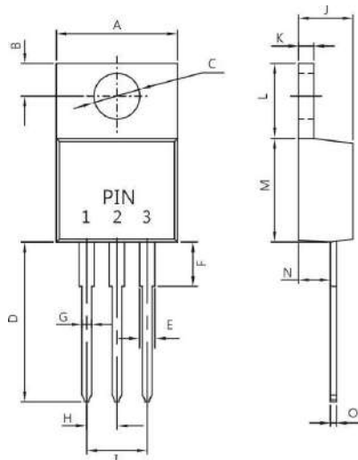
TO-220AB
