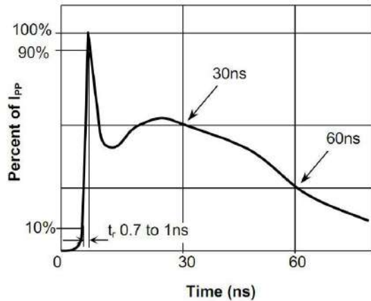
Fig.1 Pulse Waveform-ESD(IEC61000-4-2)
