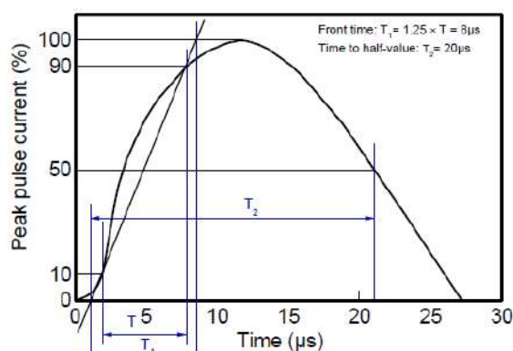
8/20 \mu s waveform per IEC61000-4-5
