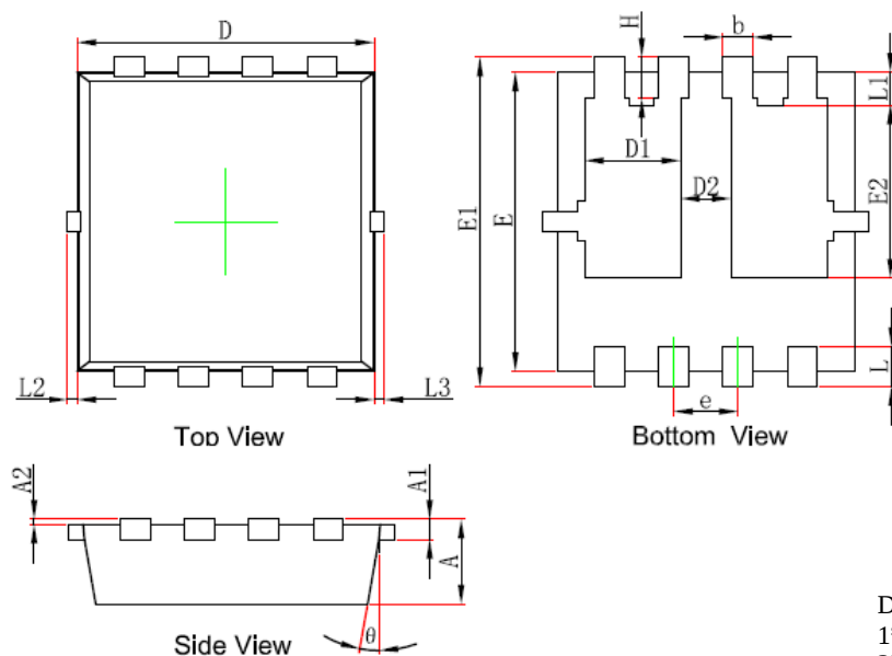
8-Lead DFN3x3 Plastic Package
