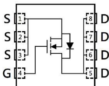
KPRE6D8N08R
