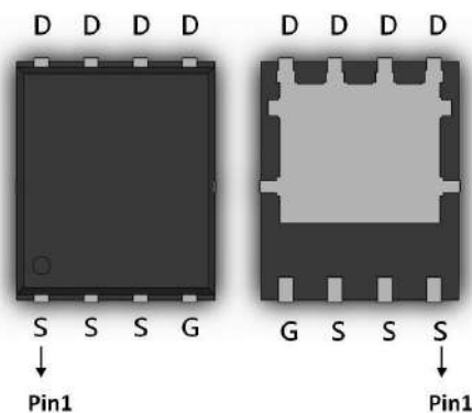
DFN5x6
