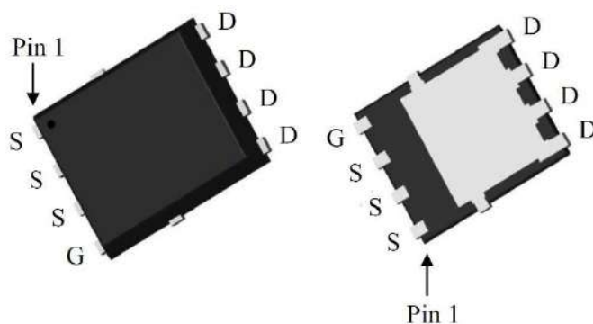
DFN5×6
