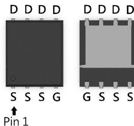
DFN5x6
