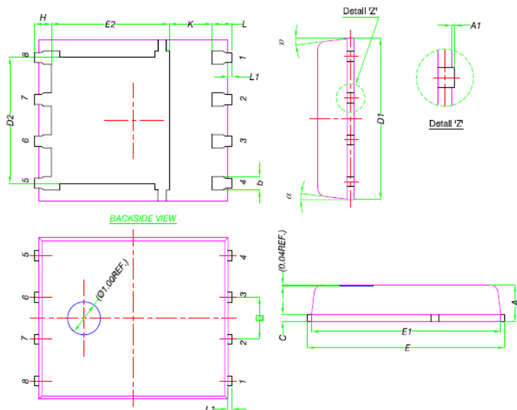
8-Lead DFN5×6 Plastic Package
