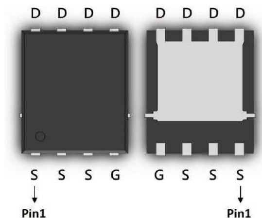
DFN5x6
