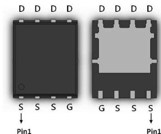
DFN5x6
