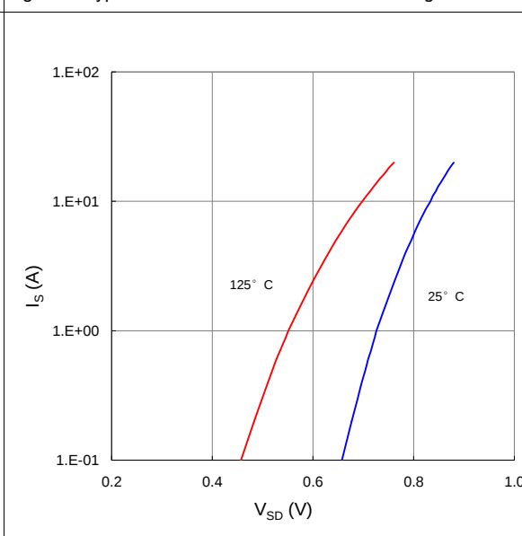
Figure 6. Typical Source-Drain Diode Forward Voltage
