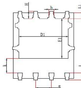
Bottom View [背视图]
