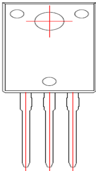
BOTTOM VIEW
