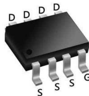
SOP8 Pin Configuration
