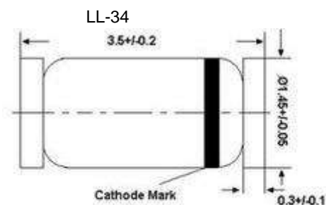
Glass case MiniMELF Dimensions in mm
