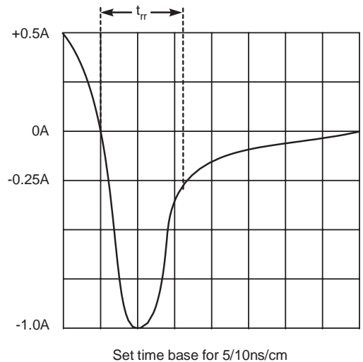
5 Reverse Recovery Time Characteristic and Test Circuit
