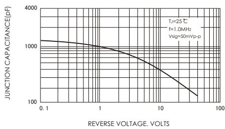
FIG.5-TYPICAL JUNCTION CAPACITANCE
