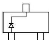
BAS40W MARKING: 43•
