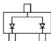
BAS40W-06 MARKING: 46
