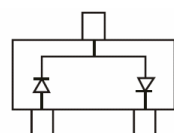
BAS40-04T MARKING:44
