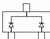
BAS40-05T MARKING:45
