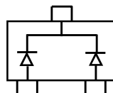
BAS70W-05 Marking: K75
