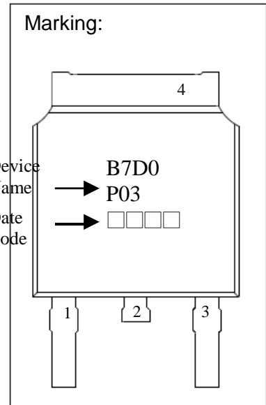
Style: Pin 1.Gate 2.Drain 3.Source 4.Drain
