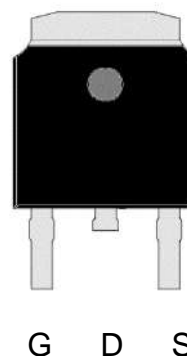
TO-252
