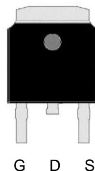
TO-252
