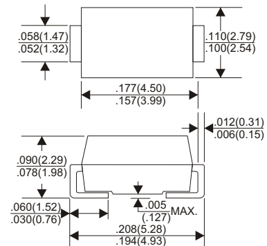
DO-214AC
