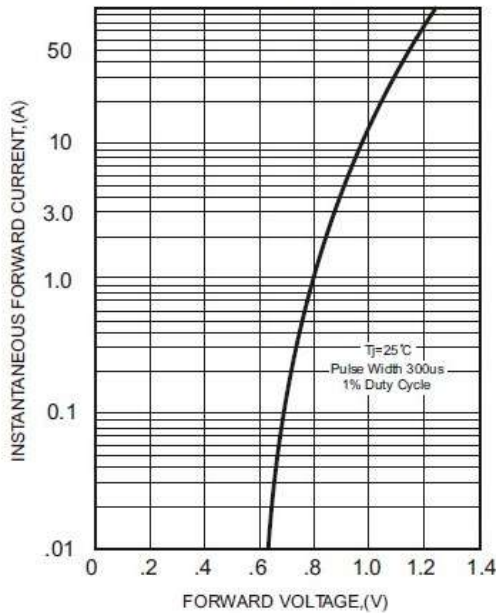
FIG.3-TYPICAL FORWARD CHARACTERISTICS
