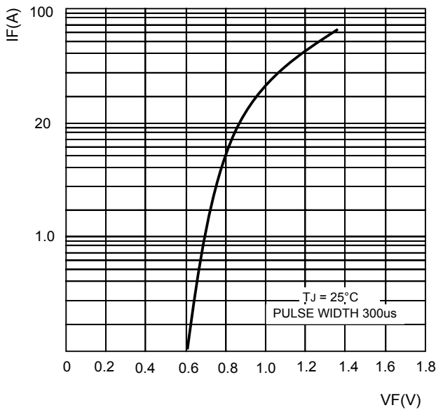
FIG.3-TYPICAL FORWARD CHARACTERISTICS
