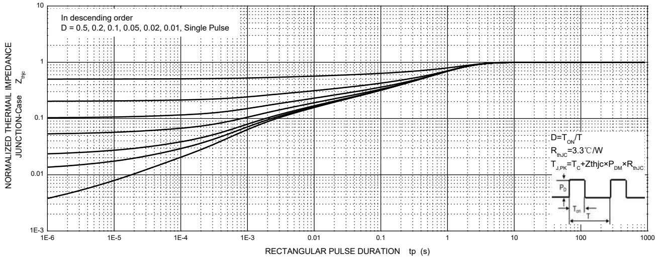
MURF1560 Transient Thermal Impedance, Junction-Case
